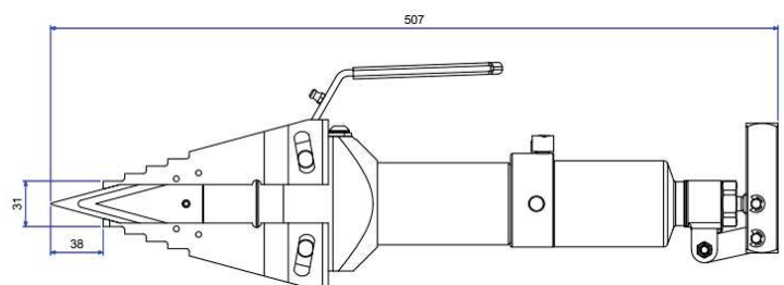
TOOL DIMENSIONS - OPEN
