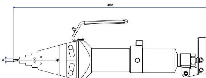
TOOL DIMENSIONS - CLOSED
